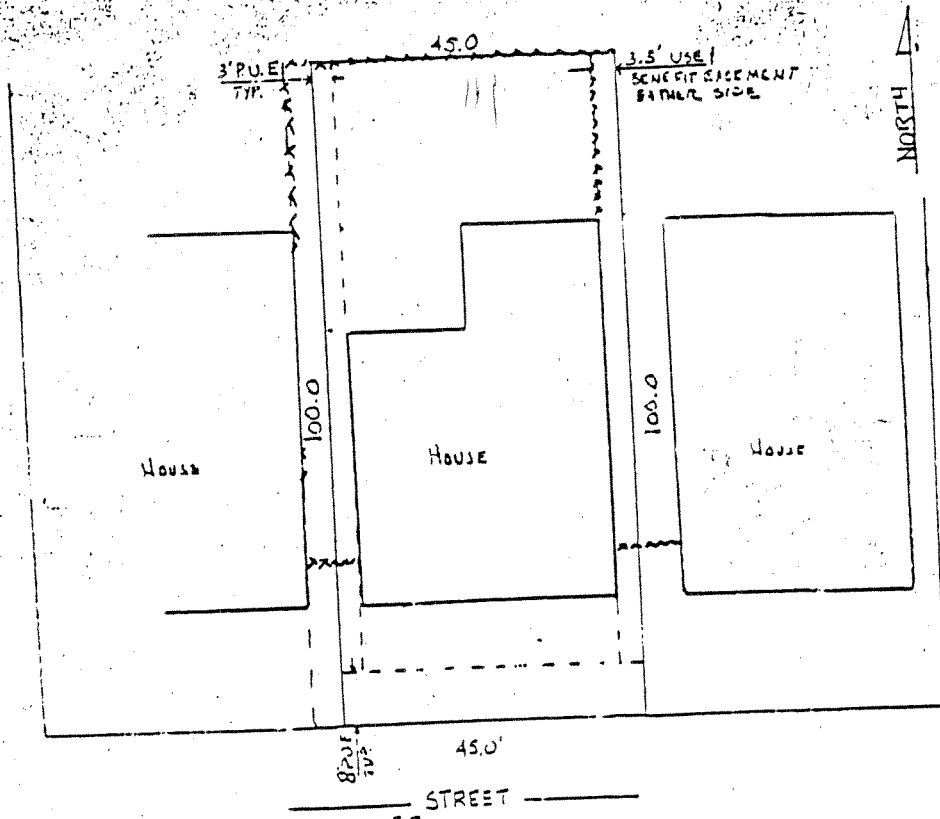
TYPICAL PLOT PLAN
